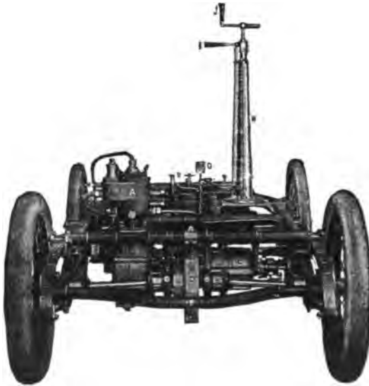
FIG. 387.—Rear view of the Running Gear and Mechanism of the Typical De Dion Carriage. A is the motor; B , the vaporizer or carburetter; C , the change speed gear; D , the differential gear, connecting to the universal jointed axle, described in connection with Fig. 80; F , the curved axle bar for maintaining rigid relations between the drive wheels; G , the pedal connecting to the auxiliary brake; H , the combined steering and control column; I , the variable speed control and brake handle; J , the steering handle.
